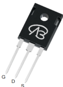
TO-247
